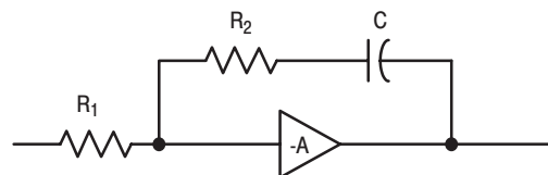
Figure 9. Active Filter Design
