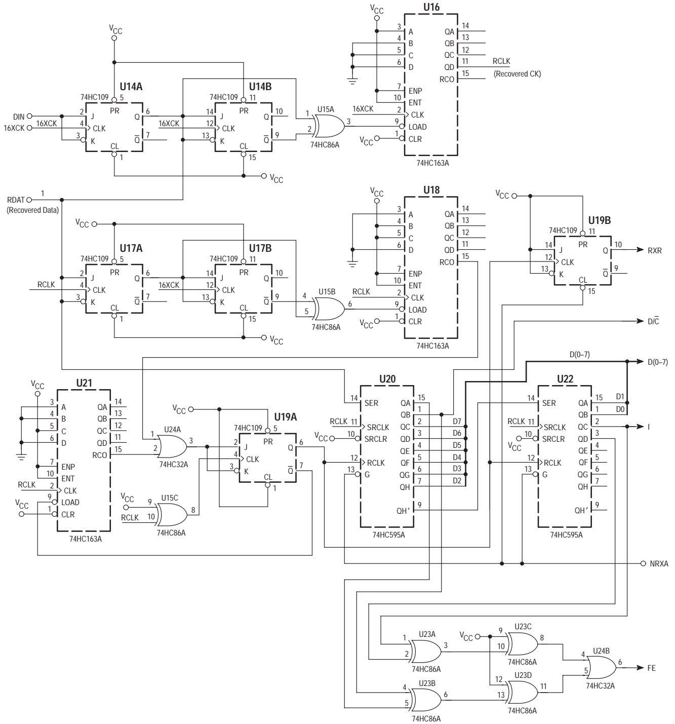
Figure 8. Decoder
