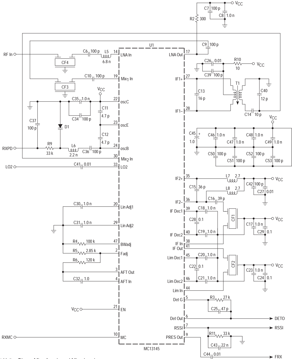
Figure 2. RF Receiver
